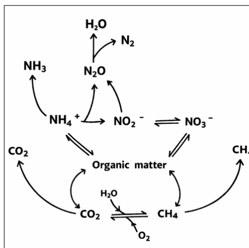
Figure 1. Production of GHG (i.e. \text{CH}_4 , \text{CO}_2 , and \text{N}_2\text{O} ) during composting [Cui et al., 2025]
